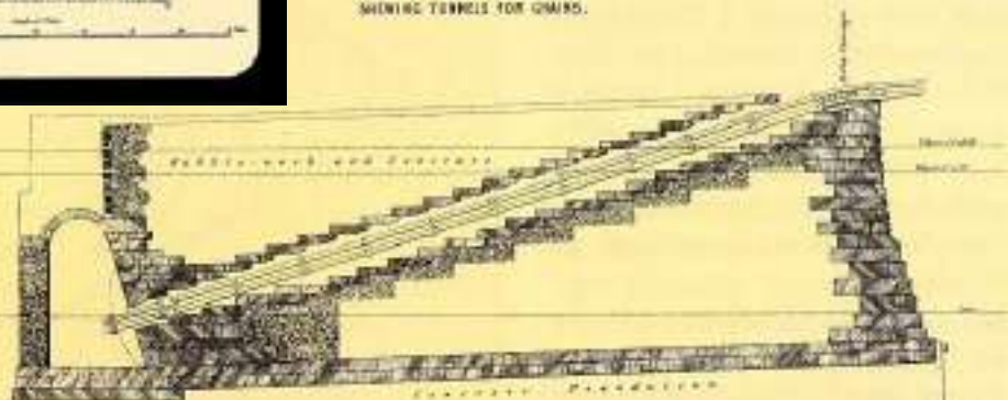
LONGITUDINAL SECTION OF FUTURE PIER, SHOWING TUNNELS FOR CARS.
